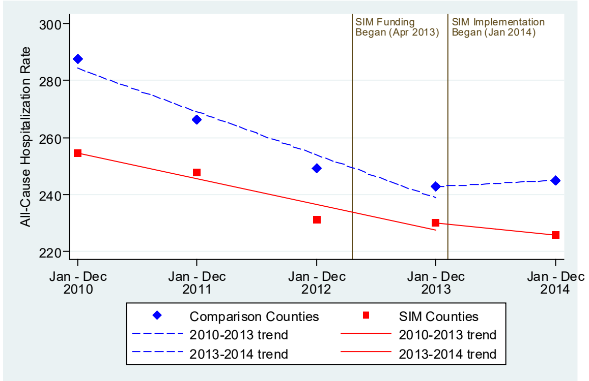
Figure A4: Unadjusted, Mean All-Cause Hospitalization Rate per 1000 Adults Diagnosed with Diabetes in SIM versus Comparison Counties, 2010-2014
