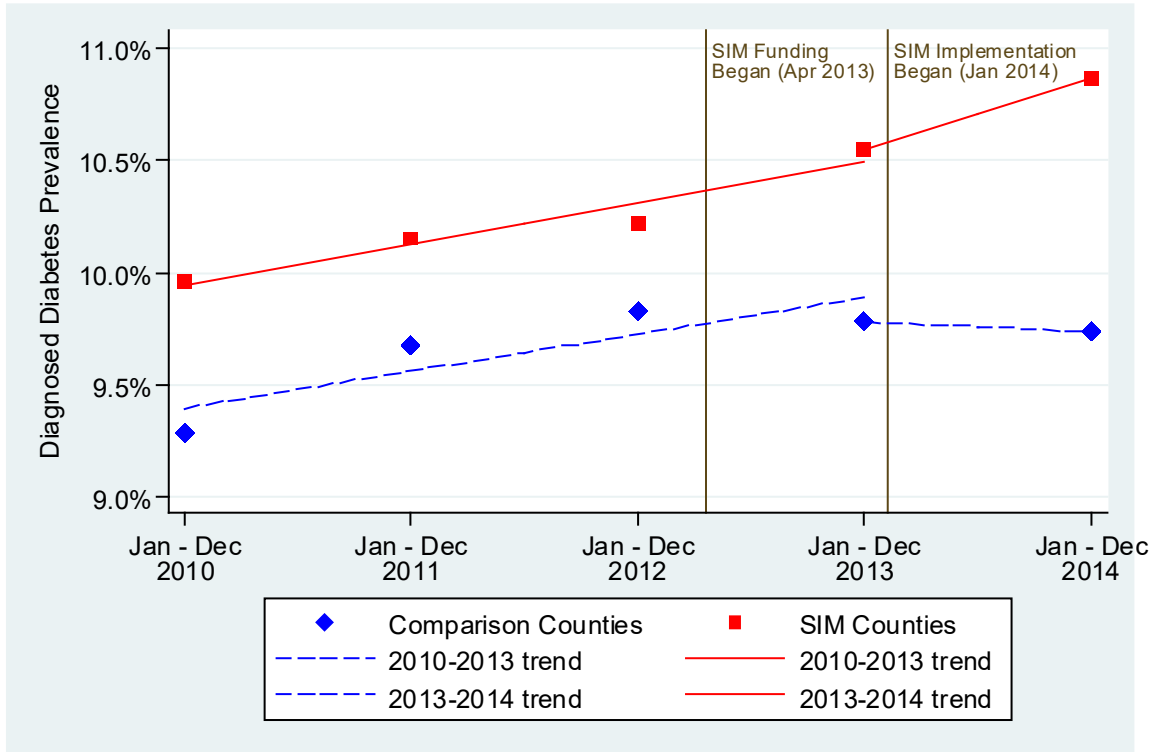
Figure A2: Unadjusted, Mean Diagnosed Diabetes Prevalence among Adults in SIM versus Comparison Counties, 2010-2014
