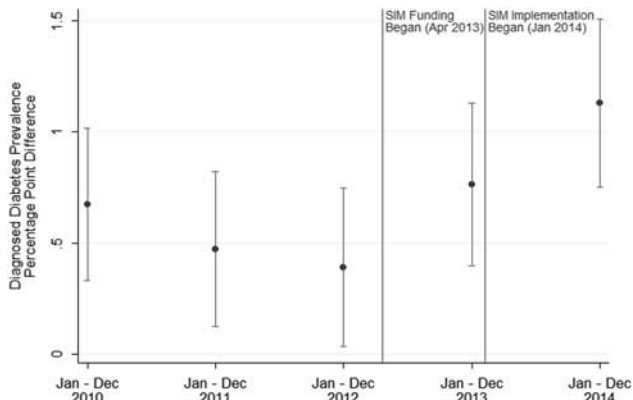
FIGURE 1. Unadjusted, mean differences in diagnosed diabetes prevalence among adults for SIM versus comparison counties, 2010–2014. SIM funding began on Apr 1, 2013, which included an initial 6-month test period, resulting in the test implementation phase beginning Oct 1, 2013. Because the diagnosed diabetes prevalence data is annual, we modeled the implementation period as beginning Jan 1, 2014. Prevalence differences were calculated each year by subtracting the mean of the county-level prevalence in the 240 SIM counties from the mean of the county-level prevalence in the 343 comparison counties. The error bars are 95% confidence intervals of the difference in the mean prevalence by year. Apr indicates April; Dec, December; Jan, January; Oct, October; SIM, State Innovation Models. Source: Authors’ analysis of Centers for Disease Control and Prevention’s county-level estimates.
