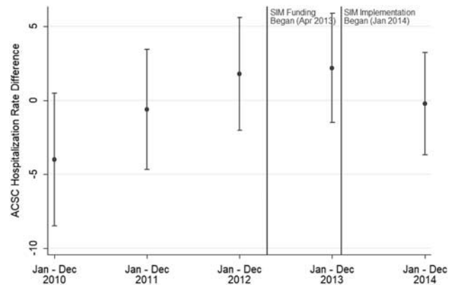
FIGURE 2. Unadjusted, mean differences in ACSC hospitalization rate per 1000 adults diagnosed with diabetes for SIM versus comparison counties, 2010–2014. SIM funding began on Apr 1, 2013, which included an initial 6-month test period, resulting in the test implementation phase beginning Oct 1, 2013. Because the diagnosed diabetes prevalence data is annual, we modeled the implementation period as beginning Jan 1, 2014. Hospital rate differences were calculated each year by subtracting the mean of the county-level hospitalization rate in the 240 SIM counties from the mean of the county-level hospitalization rate in the 343 comparison counties. The error bars are 95% confidence intervals of the difference in the mean hospitalization rate by year. ACSC indicates ambulatory care-sensitive condition; Apr, April; Dec, December; Jan, January; Oct, October; SIM, State Innovation Models. Sources: Authors’ analysis of Centers for Disease Control and Prevention’s county-level estimates and Healthcare Cost and Utilization Project’s State Inpatient Databases.
