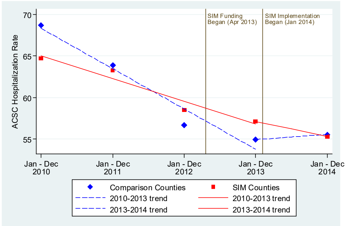
Figure A3: Unadjusted, Mean ACSC Hospitalization Rate per 1000 Adults Diagnosed with Diabetes in SIM versus Comparison Counties, 2010-2014
