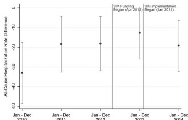
FIGURE 3. Unadjusted, mean differences in all-cause hospitalization rate per 1000 adults diagnosed with diabetes for SIM versus comparison counties, 2010–2014. SIM funding began on Apr 1, 2013, which included an initial 6-month test period, resulting in the test implementation phase beginning Oct 1, 2013. Because the diagnosed diabetes prevalence data is annual, we modeled the implementation period as beginning Jan 1, 2014. Hospital rate differences were calculated each year by subtracting the mean of the county-level hospitalization rate in the 240 SIM counties from the mean of the county-level hospitalization rate in the 343 comparison counties. The error bars are 95% confidence intervals of the difference in the mean hospitalization rate by year. Apr indicates April; Dec, December; Jan, January; Oct, October; SIM, State Innovation Models. Sources: Authors' analysis of Centers for Disease Control and Prevention's county-level estimates and Healthcare Cost and Utilization Project's State Inpatient Databases.
